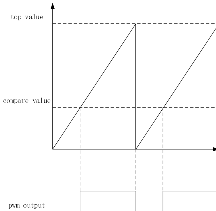
Figure 15: PWM operation
