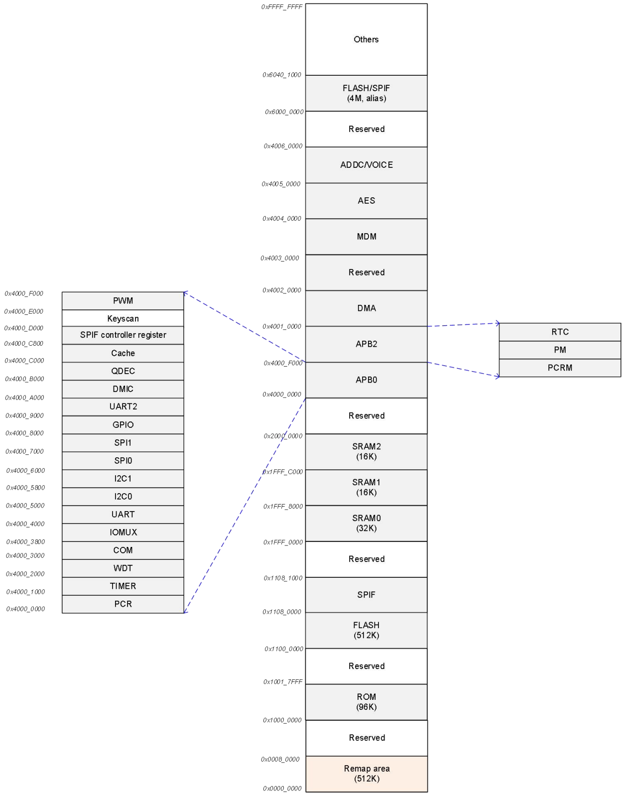
Figure 3: TG7120B-OB memory space
