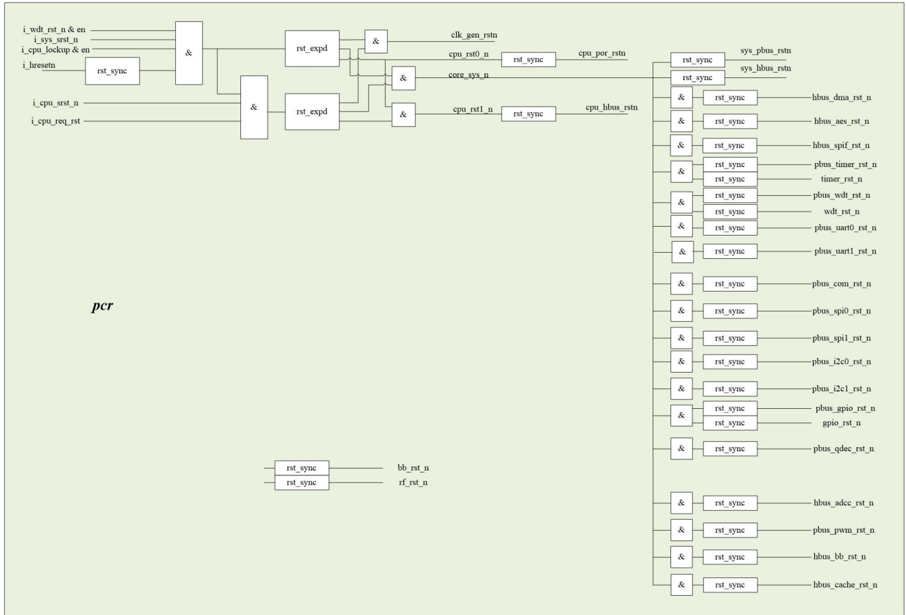
Figure 6: TG7120B-OB power, clock and reset
