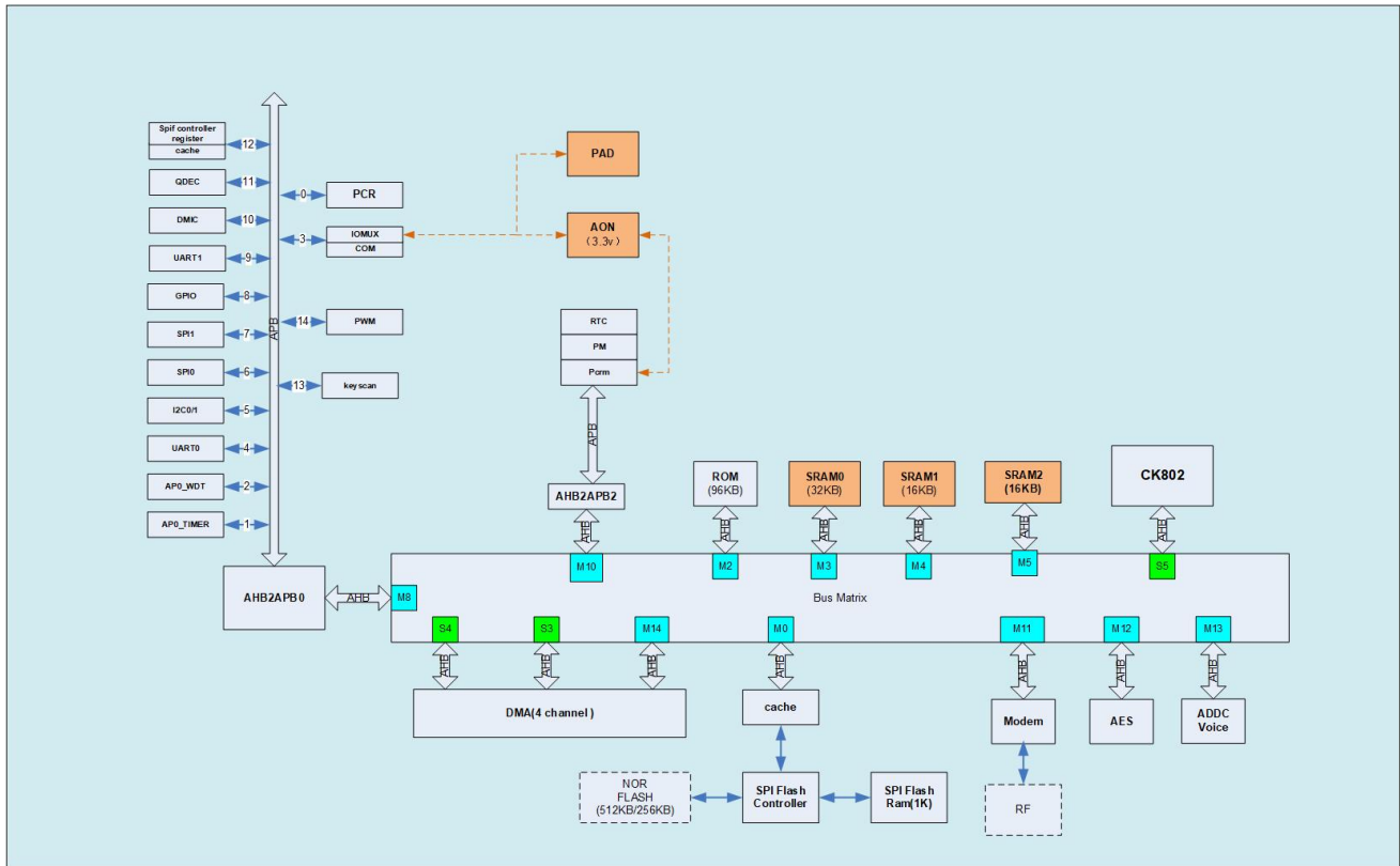
Figure 1: TG7120B-OB block diagram
