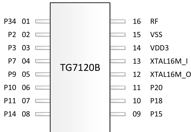
Figure 2: Pin assignment – TG7120B-OB SOP16 package
