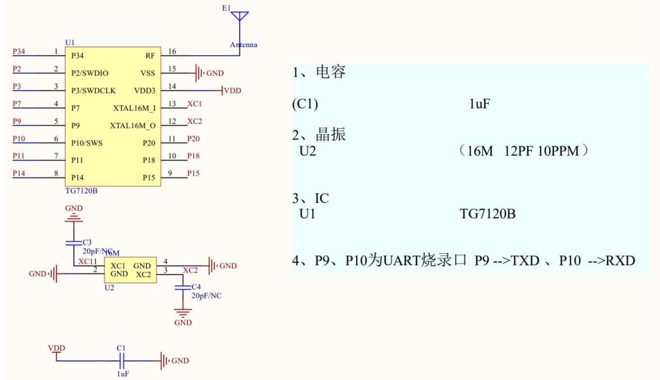
Figure 19: Sample application of SOP16
