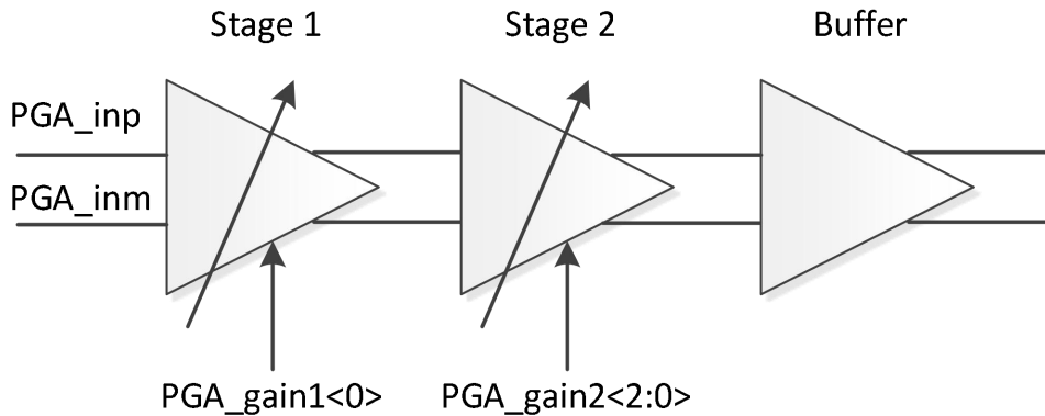
Figure 17: PGA path
