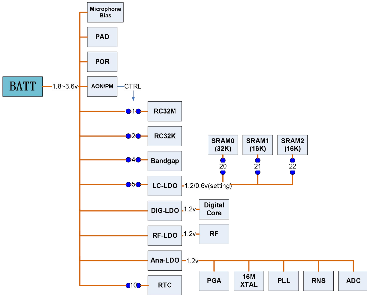
Figure 7: Power system
