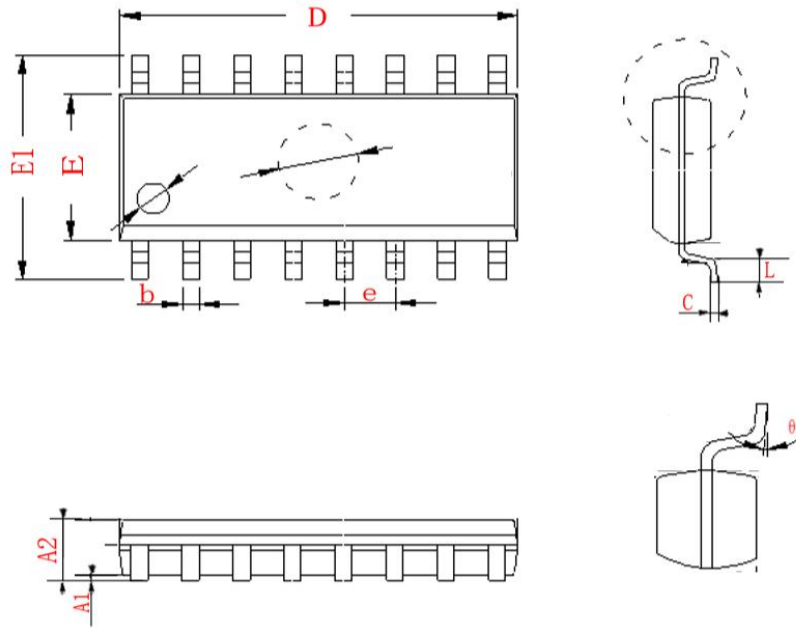
Figure 18: SOP16 package dimensions
