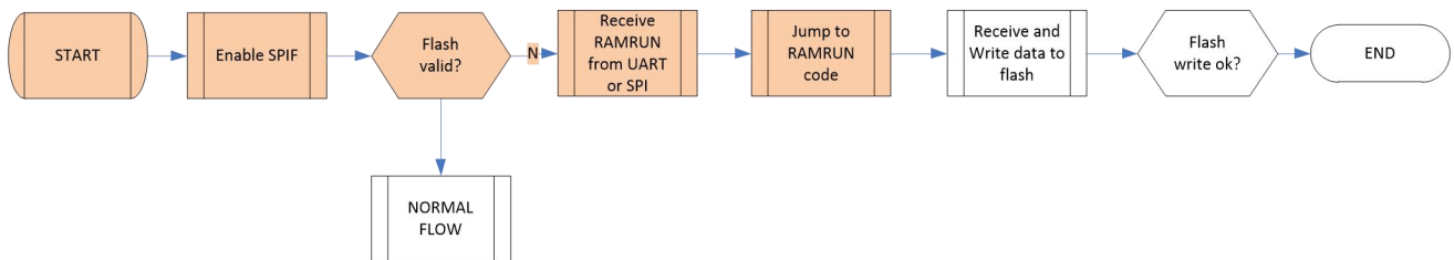
Figure 5: Bootloader flow
