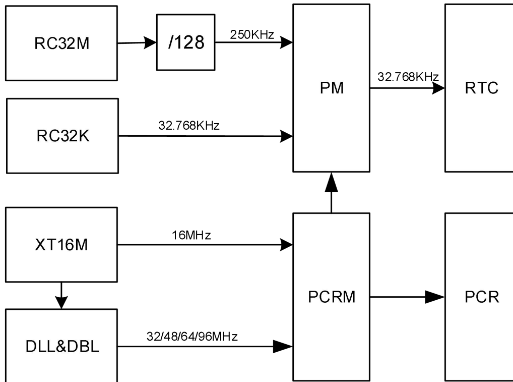
Figure 9: Clock management
