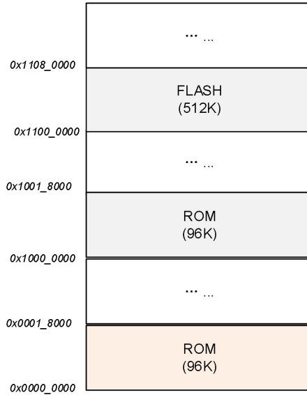
Figure 4: TG7120B-OB boot mode
